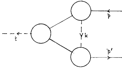
FIG. 5. Basic triangle graph for the vertex equation.
