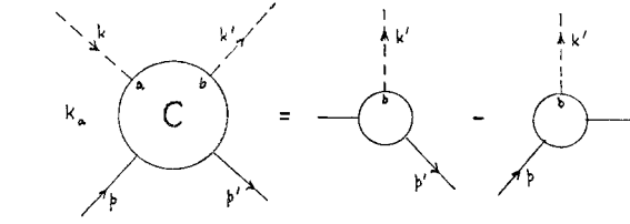
FIG. 6. Diagrammatic interpretation of the gauge identity for proper Compton scattering.
