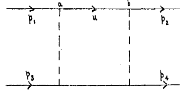
FIG. 3. Meson-meson scattering.
